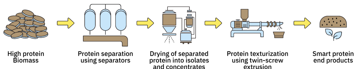
Figure 1. Equipment-driven production flow for plant-based smart protein manufacturing
