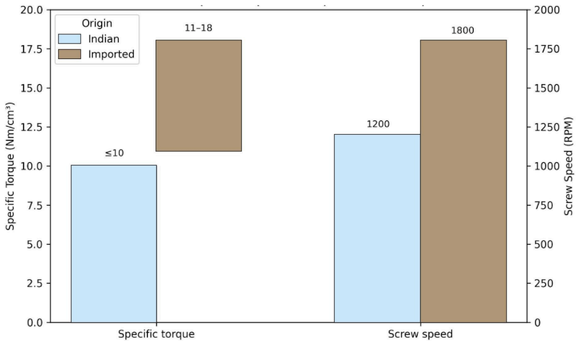
Figure 9. Indian vs. imported extruders: Specific torque and screw speed
